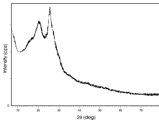
Figure 2 X-ray diffraction pattern of PANI-phosphate pigment.
