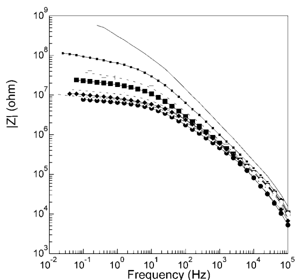
Figure 5 Impedance plots of PANI-phosphate pigmented epoxy coated AA2024-T3 alloy in 0.5% NaCl; — Initial; ■ 1 day; □ 4 days; ■ 7 days; ○ 15 days; ● 28 days; ◇ 38 days; ◆ 50 days.
