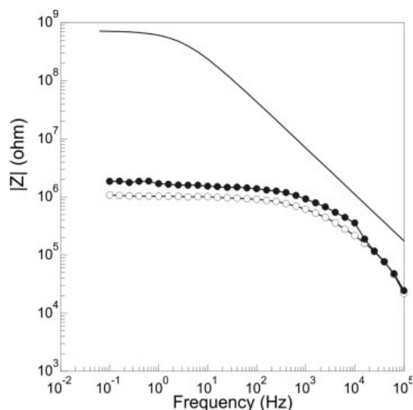
Figure 6 Impedance plots of strontium chromate pigmented acrylic coated A2024-T3 alloy in 0.5% NaCl; — Initial; ○ 15 days; ● 28 days.
