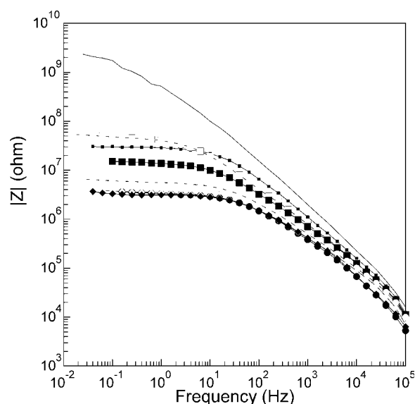
Figure 4 Impedance plots of PANI-phosphate pigmented acrylic coated AA2024-T3 alloy in 0.5% NaCl; — Initial; ■ 1 day; □ 4 days; ■ 7 days; ○ 15 days; ● 28 days; ◇ 38 days; ◆ 50 days.
