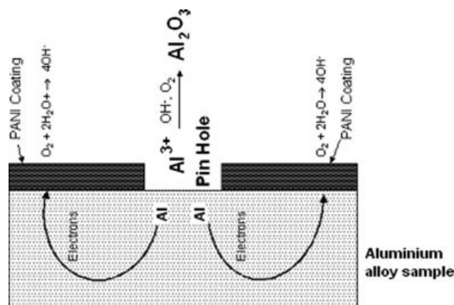
Figure 7 Schematic diagram of mechanism of AA2024-T3 alloy passivation by PANI-blended paint coating.
