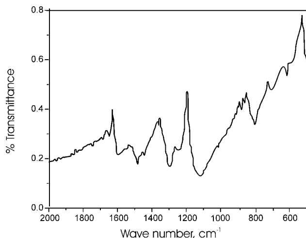
Figure 1 FTIR spectrum of PANI-phosphate pigment.
